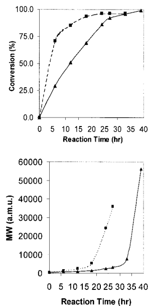
Figure 1. Polymerization kinetics for monomer 4 from GPC monitoring: (▲) dioxane, 65 °C, \text{Me}_4\text{NOH} ; (■) dioxane, 65 °C, \text{Bu}_4\text{NBr} .
